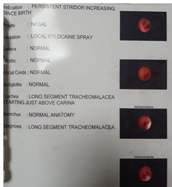
Fig. 4: Bronchoscope
