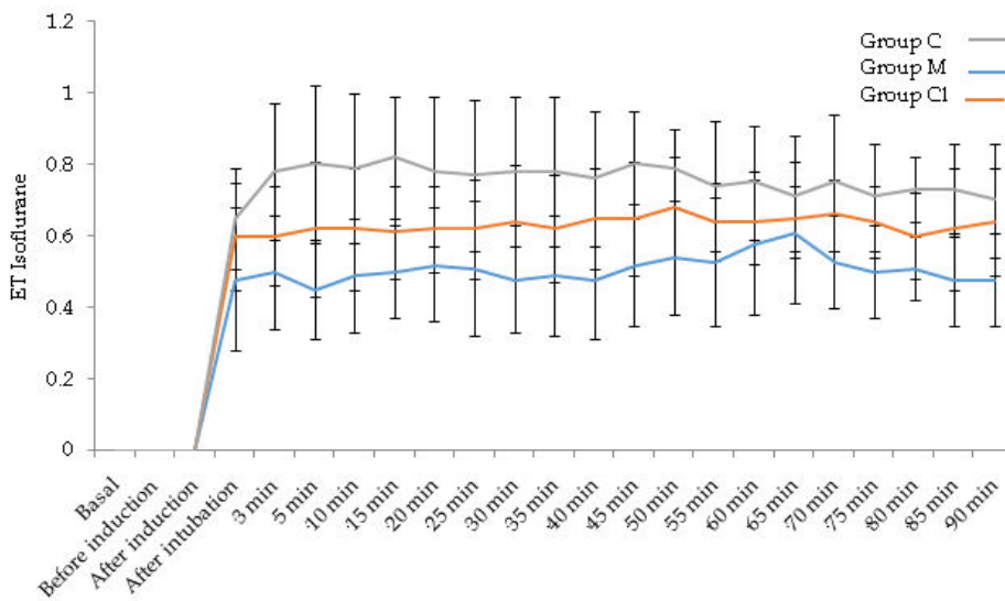
Fig. 4: Comparison of end tidal isoflurane concentration between the three groups.
