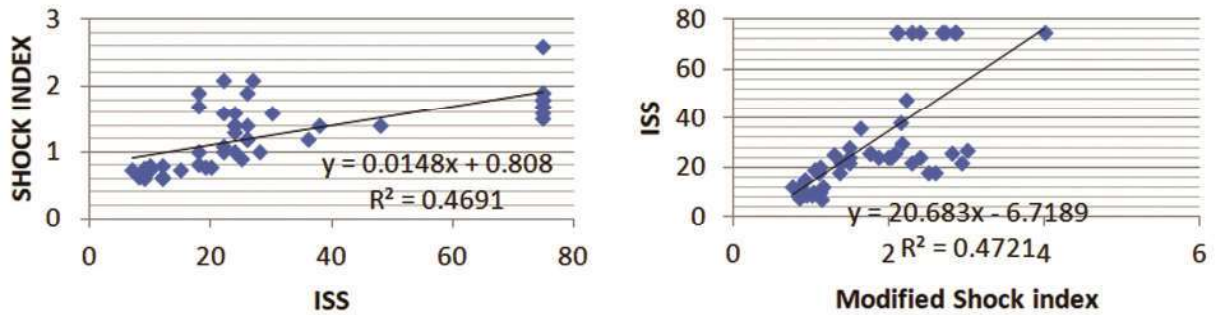
Fig. 3: Scatter Diagram Showing Correlation Between ISS & SI/MSI.
