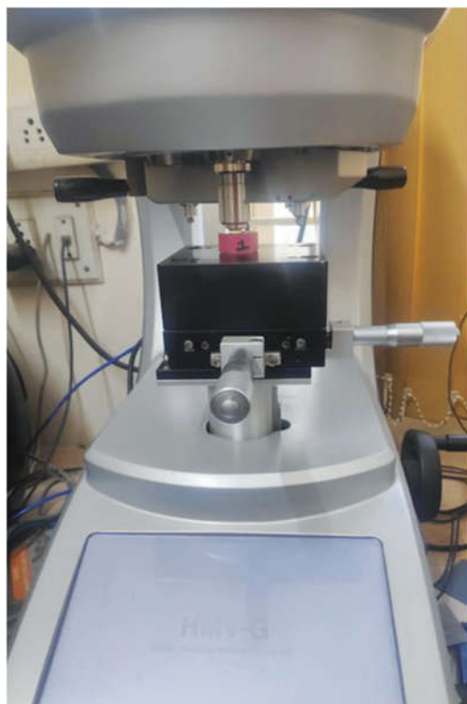
Fig. 3: Vicker's Microhardness Testing.
