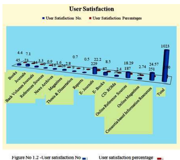
Fig. 1.2: User Satisfaction.
