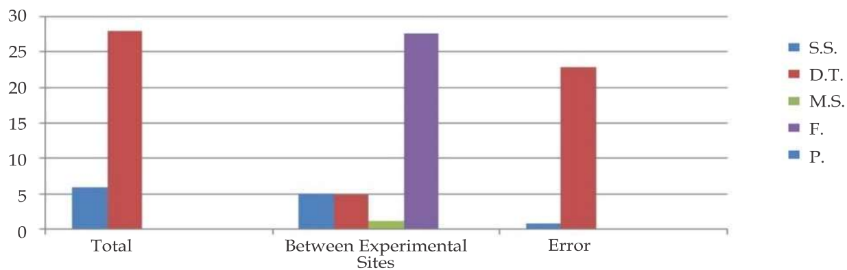
Fig 3: ANOVA of Cu/Zn SOD of data
